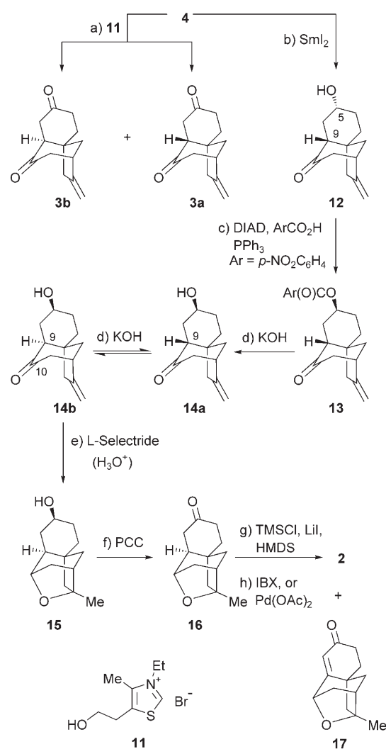
Scheme 3. Synthesis of tetracyclic enone 2 . Reagents and conditions: a) 11 (0.2 equiv), \text{Et}_3\text{N} (1.2 equiv), EtOH, 80^\circ\text{C} , 18 h, 65% ( 3a/3b ca. 5:1); b) \text{SmI}_2 (0.1 M in THF, 2.2 equiv), MeOH (2.5 equiv), 23^\circ\text{C} , THF (0.032 M), 2 min, 57%; c) p -nitrobenzoic acid (1.5 equiv), \text{PPh}_3 (1.5 equiv), DIAD (3.4 equiv), benzene, 23^\circ\text{C} , 2 h, 67%; d) KOH (10% in MeOH), 50^\circ\text{C} , 5 h, 14a : 46%, 14b : 45%; e) L-selectride (1.0 M in THF, 4.0 equiv), THF, -78 \rightarrow 23^\circ\text{C} , 2 h; then 1 M aq HCl, 0 \rightarrow 23^\circ\text{C} , 2 h, 80%; f) PCC (2.0 equiv), \text{CH}_2\text{Cl}_2 , 23^\circ\text{C} , 1.5 h, 95%; g) TMSCl (3.3 equiv), Lil (3.3 equiv), HMDS (5.0 equiv), \text{CH}_2\text{Cl}_2 , 0^\circ\text{C} , 3 h; h) 1. IBX (1.5 equiv), MPO (1.5 equiv), DMSO, 23^\circ\text{C} , 2 h, 2 : 53%, 17 : 26%; or 2. \text{Pd}(\text{OAc})_2 (1.0 equiv), \text{CH}_3\text{CN} , 23^\circ\text{C} , 5 h, 2 : 60%, 17 : 30%; DIAD = diisopropyl azodicarboxylate; IBX = o -iodoxybenzoic acid; MPO = 4-methoxy-pyridine- N -oxide.
